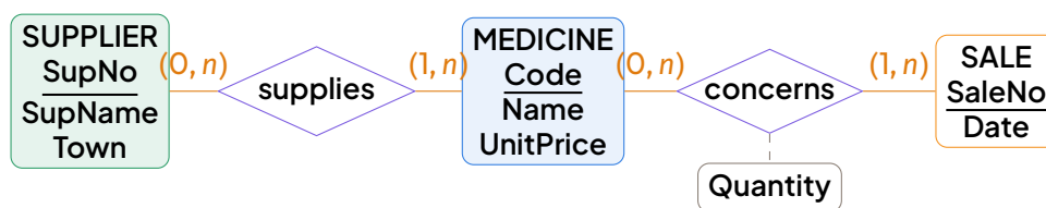
ER diagram of the pharmacy database (identifiers underlined).
