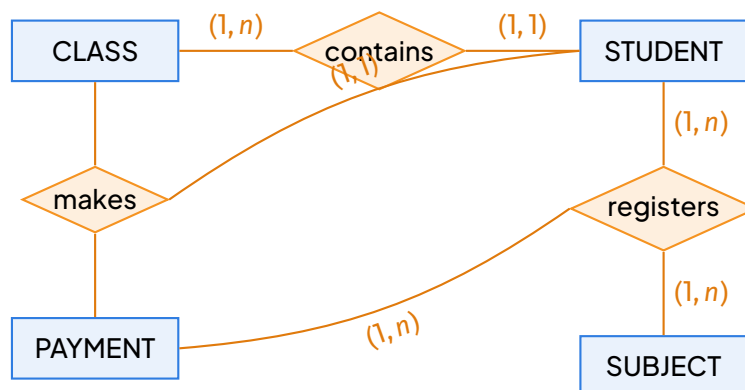
ER diagram of SchoolManager: four entities and three relationships with their cardinalities.
