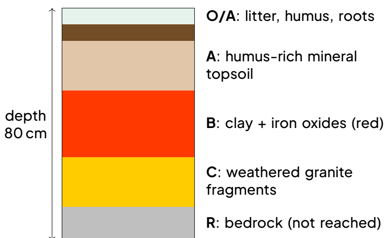
Labelled sketch of the school soil pit (idealised profile of a ferrallitic soil).
