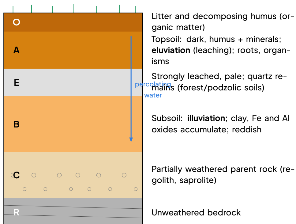
Idealised soil profile showing the master horizons O, A, E, B, C and R, with their typical colours, compositions and dominant processes.
