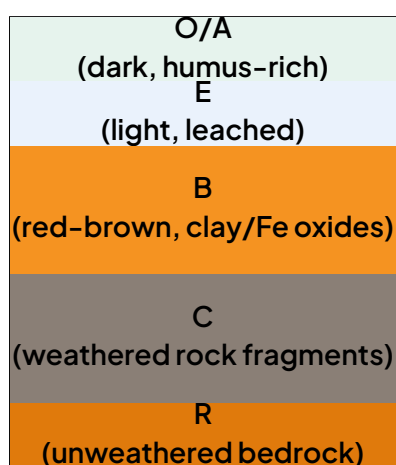
Idealised soil profile showing horizon sequence O/A–E–B–C–R.
