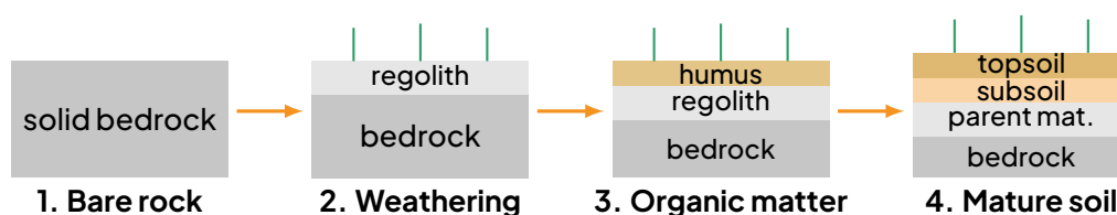
Schematic sequence of the four stages of soil formation, from bare bedrock to a mature, layered soil.
