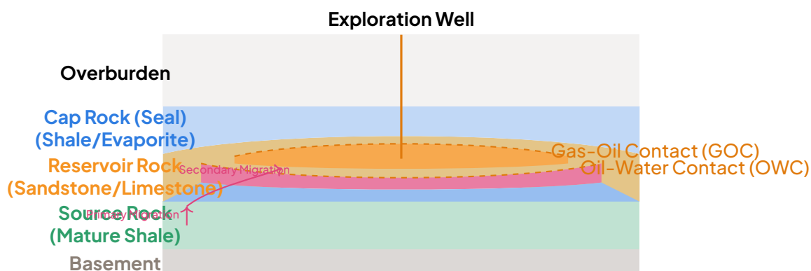
Cross-section of an anticlinal trap. Note the fluid contacts (GOC, OWC) are horizontal (gravity equilibrium), while the rock layers are folded. The well targets the crest (culmination) for maximum hydrocarbon column.
