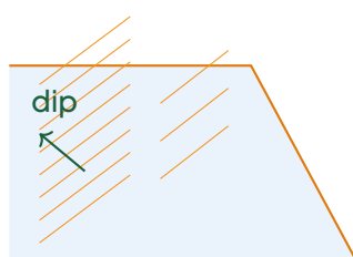
Stable: joints dip into the road cut
