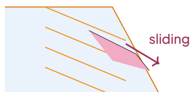
Unstable: joints dip out of the road cut
