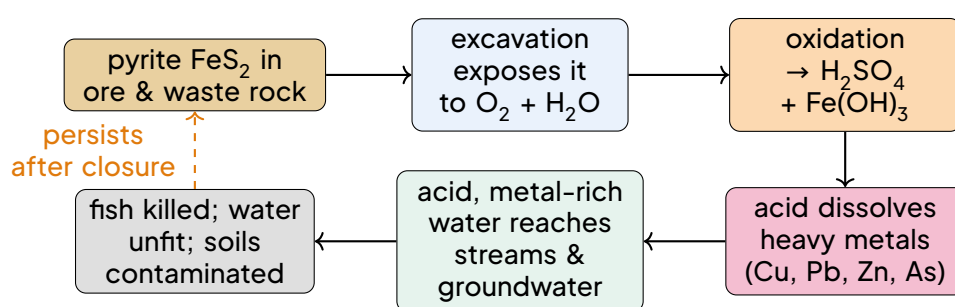
Formation of acid mine drainage from the oxidation of pyrite in exposed waste rock and abandoned workings.
