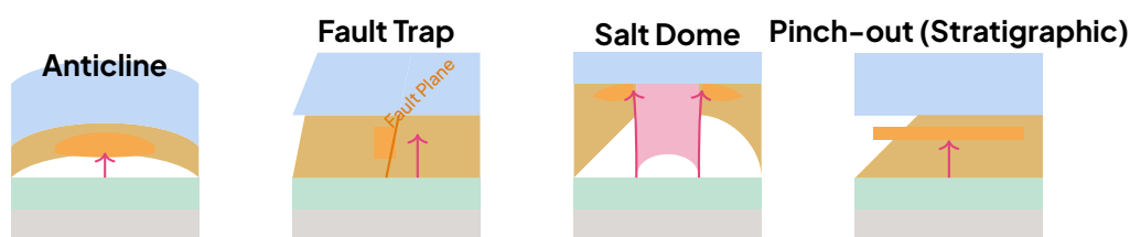
Gallery of four major trap types. (1) Anticline: structural, most common. (2) Fault trap: reservoir sealed by fault juxtaposition. (3) Salt dome: salt diapir creates flank traps. (4) Pinch-out: stratigraphic, reservoir thins into seal.
