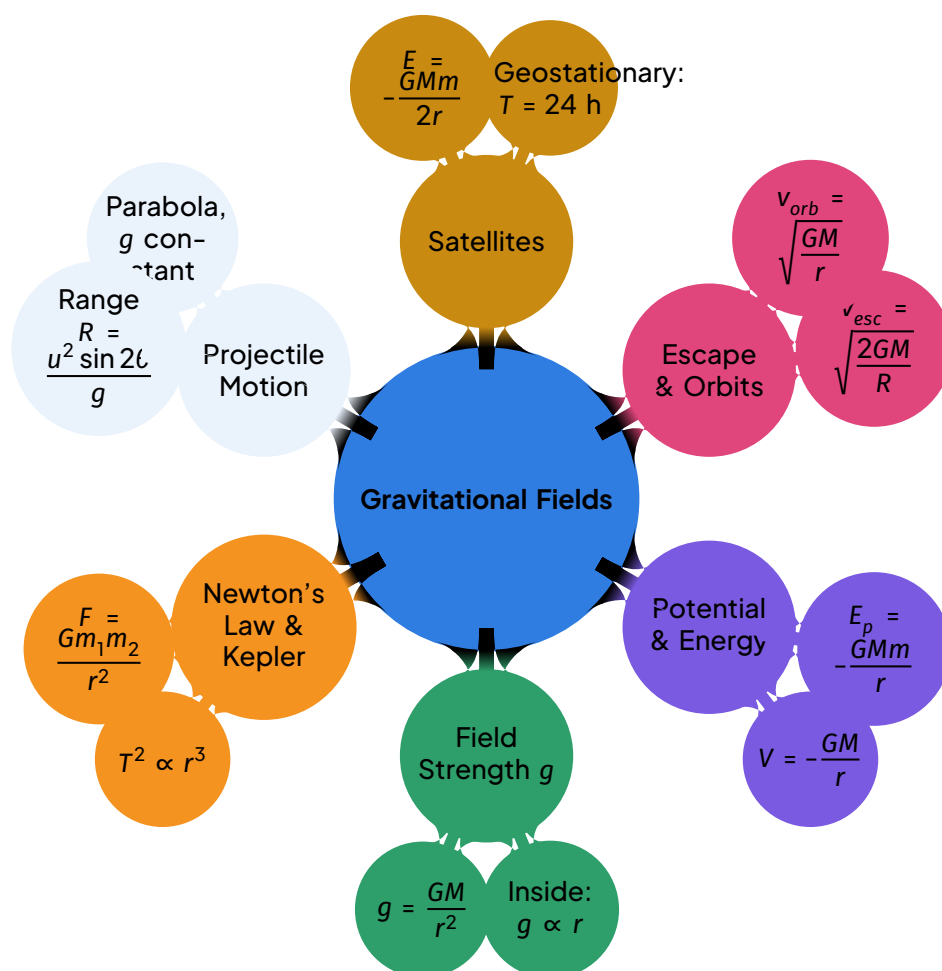
Mind map of the chapter: Gravitational Fields.
