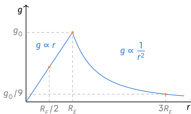
Variation of g with distance r from the centre of a uniform Earth.
