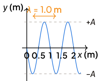
Graph of y against x at t = 0 : amplitude A = 0.04 \text{ m} , wavelength \lambda = 1.0 \text{ m} .
