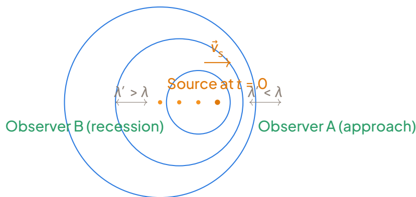
Wavefronts emitted by a source moving to the right. Wavefronts are compressed ahead (shorter \lambda' ) and stretched behind (longer \lambda' ).
