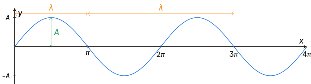
Snapshot y(x) at fixed t : the spatial period is \lambda .
