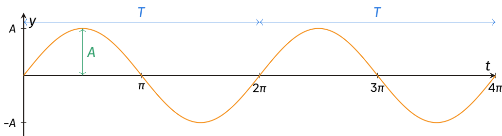
Vibration graph y(t) at fixed x : the temporal period is T .
