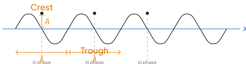
Labelled sinusoidal wave showing amplitude A , wavelength \lambda , crests and troughs. Points separated by integer multiples of \lambda are in phase.
