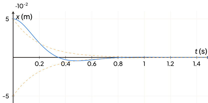
Underdamped response x(t) with exponential envelope \pm 0.05e^{-5t} .
