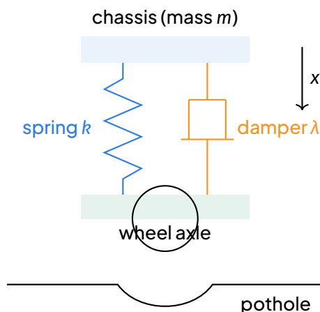
Quarter-car model of the suspension: spring and damper in parallel.
