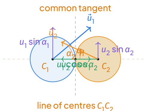
Two smooth spheres at the instant of impact: line of centres, common tangent, and each velocity resolved into components.
