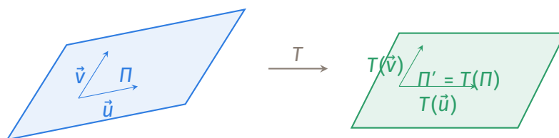
A plane \Pi spanned by \vec{u}, \vec{v} maps to the plane \Pi' spanned by T(\vec{u}), T(\vec{v}) .
