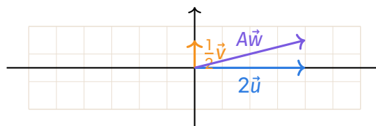
Image under A : horizontal stretch \times 2 , vertical compression \times \frac{1}{2}
