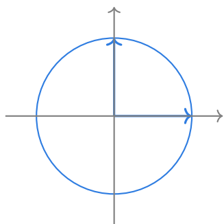
Unit circle, eigen-directions
