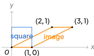
The unit square (blue) and its image under the shear (orange).
