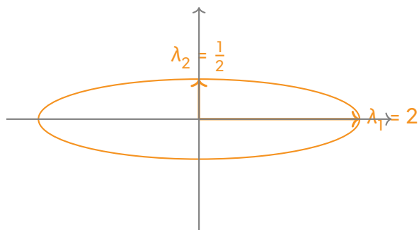
Image ellipse, axes along eigen-directions
