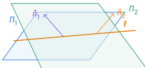
Two non-parallel planes \Pi_1 and \Pi_2 intersect along a line \ell whose direction is perpendicular to both normals \vec{n}_1 and \vec{n}_2 .
