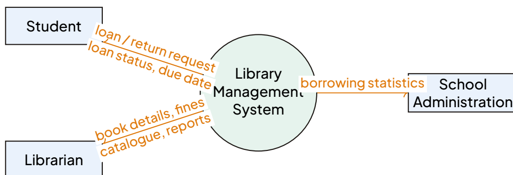
Level-0 (context) data flow diagram for a library management system: the whole system is one process exchanging data with external entities.
