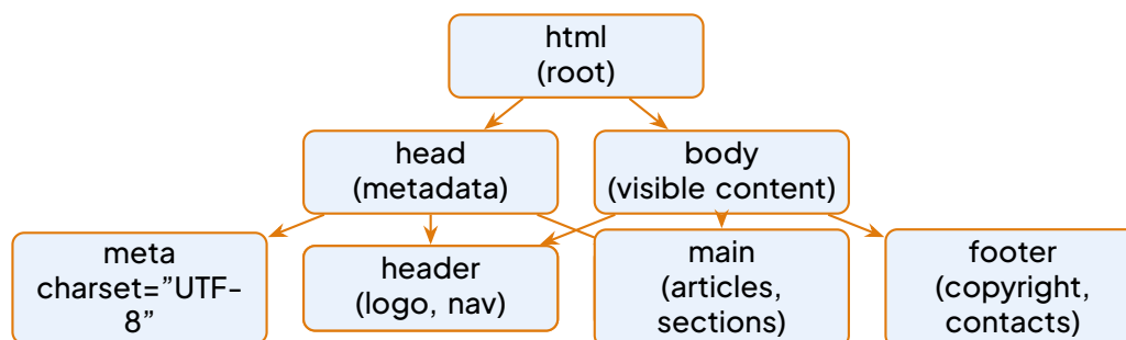
Tree diagram of the HTML document skeleton.
