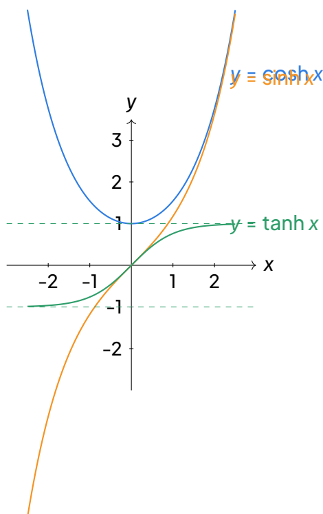
Graphs of y = \cosh x (blue), y = \sinh x (orange), y = \tanh x (green). Horizontal asymptotes y = \pm 1 for \tanh x .
