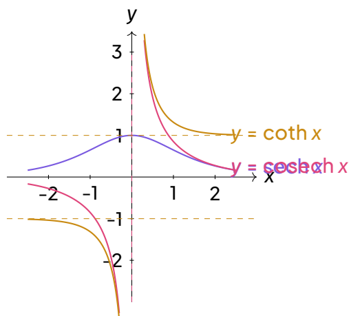
Graphs of reciprocal functions: \operatorname{sech} x (purple), \operatorname{cosech} x (pink), \coth x (gold). Vertical asymptote at x = 0 for \operatorname{cosech} x and \coth x ; horizontal asymptotes y = \pm 1 for \coth x .
