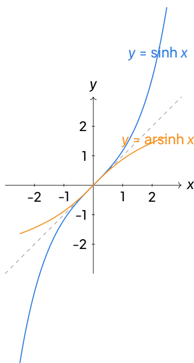
Graphs of y = \sinh x (blue) and its inverse y = \operatorname{arsinh} x (orange), symmetric about y = x .
