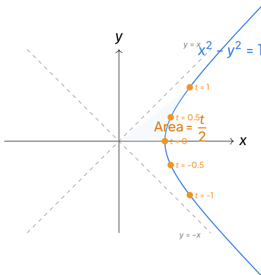
The unit hyperbola x^2 - y^2 = 1 with points (\cosh t, \sinh t) for several values of t . The shaded sector has area t/2 .
