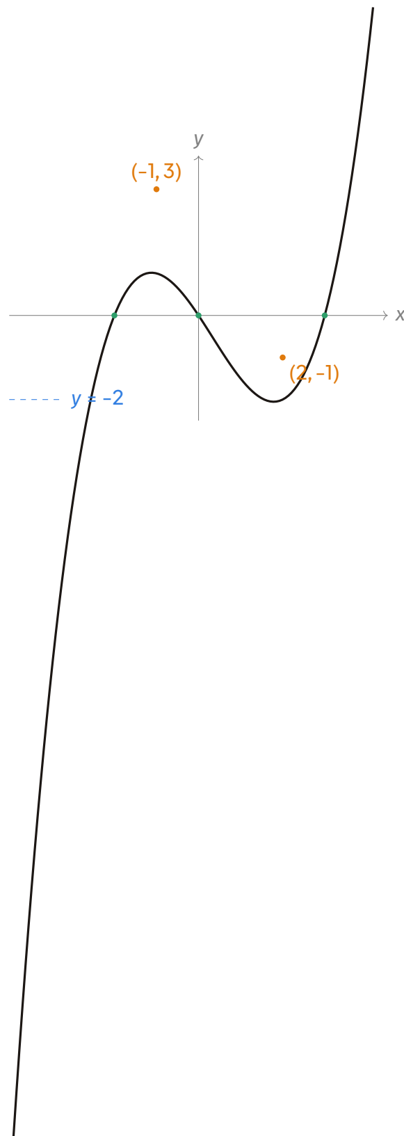
A possible qualitative curve of g satisfying the given table of variation.
