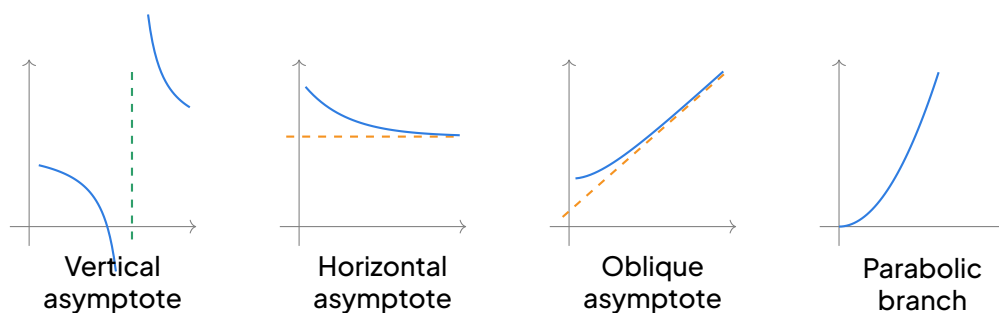
The four types of infinite branches: vertical asymptote, horizontal asymptote, oblique asymptote, parabolic branch.
