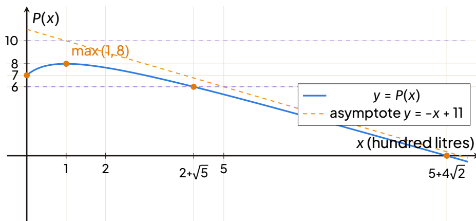
The profit curve, its oblique asymptote, and the tolerance band 6 \leq y \leq 10 .
