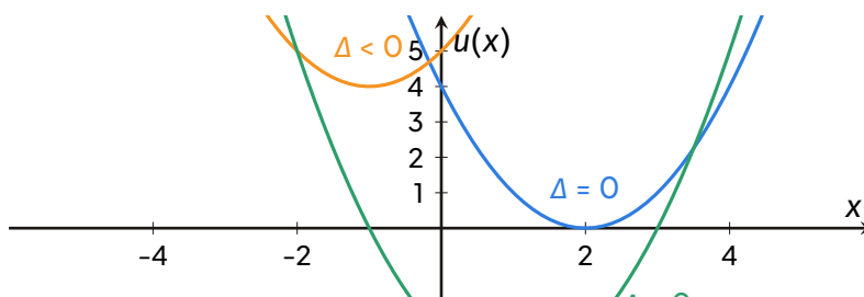
Sign of a quadratic according to its discriminant \Delta .
