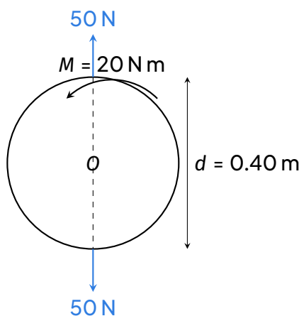
Couple on a steering wheel: equal opposite forces, moment Fd .
