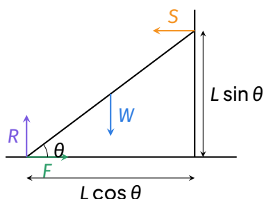
Forces on a ladder against a smooth wall
