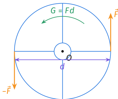
A couple applied to a steering wheel: two equal opposite tangential forces at the rim, arm d equal to the diameter, moment G = Fd .
