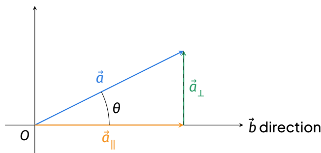
Decomposition of \vec{a} into components parallel and perpendicular to \vec{b} .
