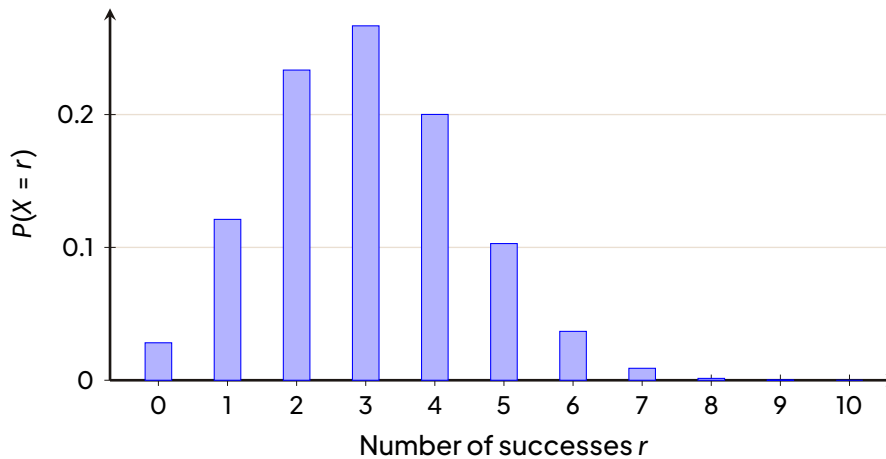
Probability mass function of X \sim B(10, 0.3) . The distribution is skewed to the right because p < 0.5 ; the most likely value is r = 3 = np .
