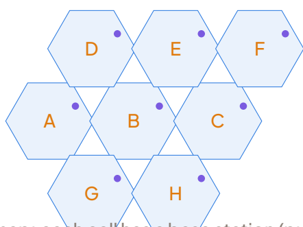
Cellular map: each cell has a base station (purple dot). Frequencies of cell A are reused in cell F, far away.
