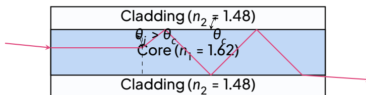
Light propagation in a step-index optical fibre by total internal reflection at the core-cladding interface.
