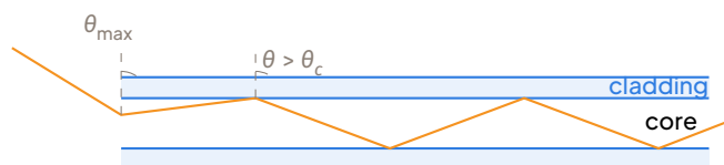
Guiding of light in a step-index fibre by total internal reflection ( n_{\text{core}} > n_{\text{cladding}} ).
