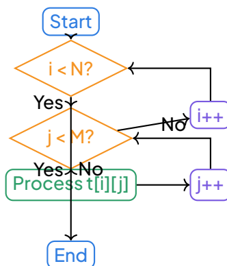
Flowchart of row-major nested loop traversal.
