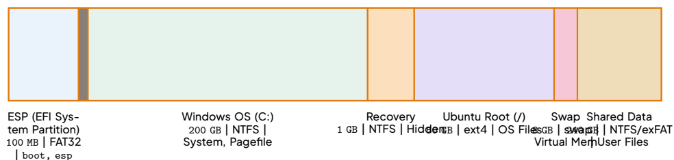
Diagram: Partitioned Hard Disk showing System, Swap, Recovery and Data Partitions (Dual-boot Windows/Ubuntu example)
