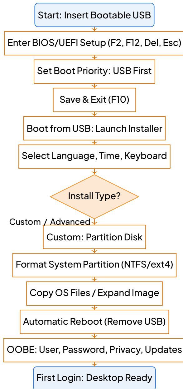
Flowchart: Typical OS Installation Process from Bootable USB to First Login
