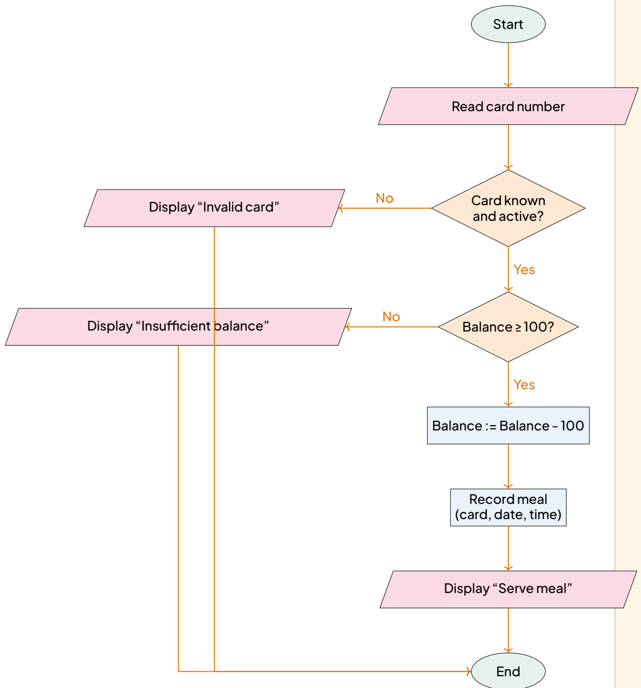
Flowchart for the "Serve a Meal" procedure
