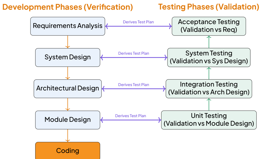
The V-Model: Linking Specification to Test
