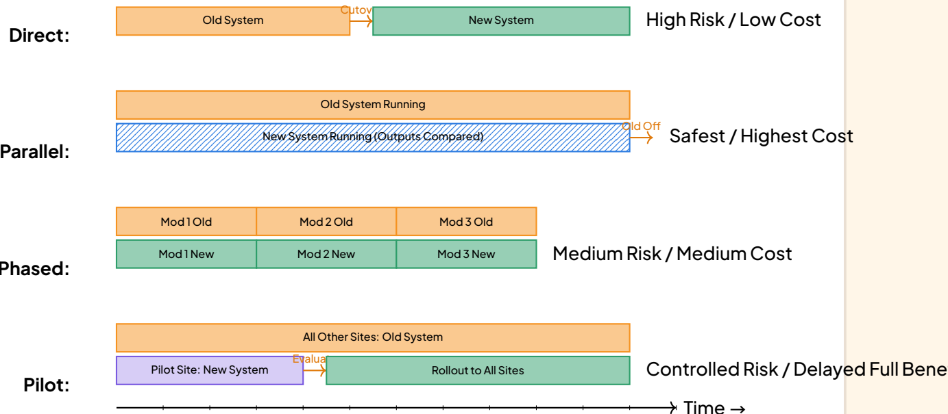
Timeline comparison of the four implementation/changeover strategies.
