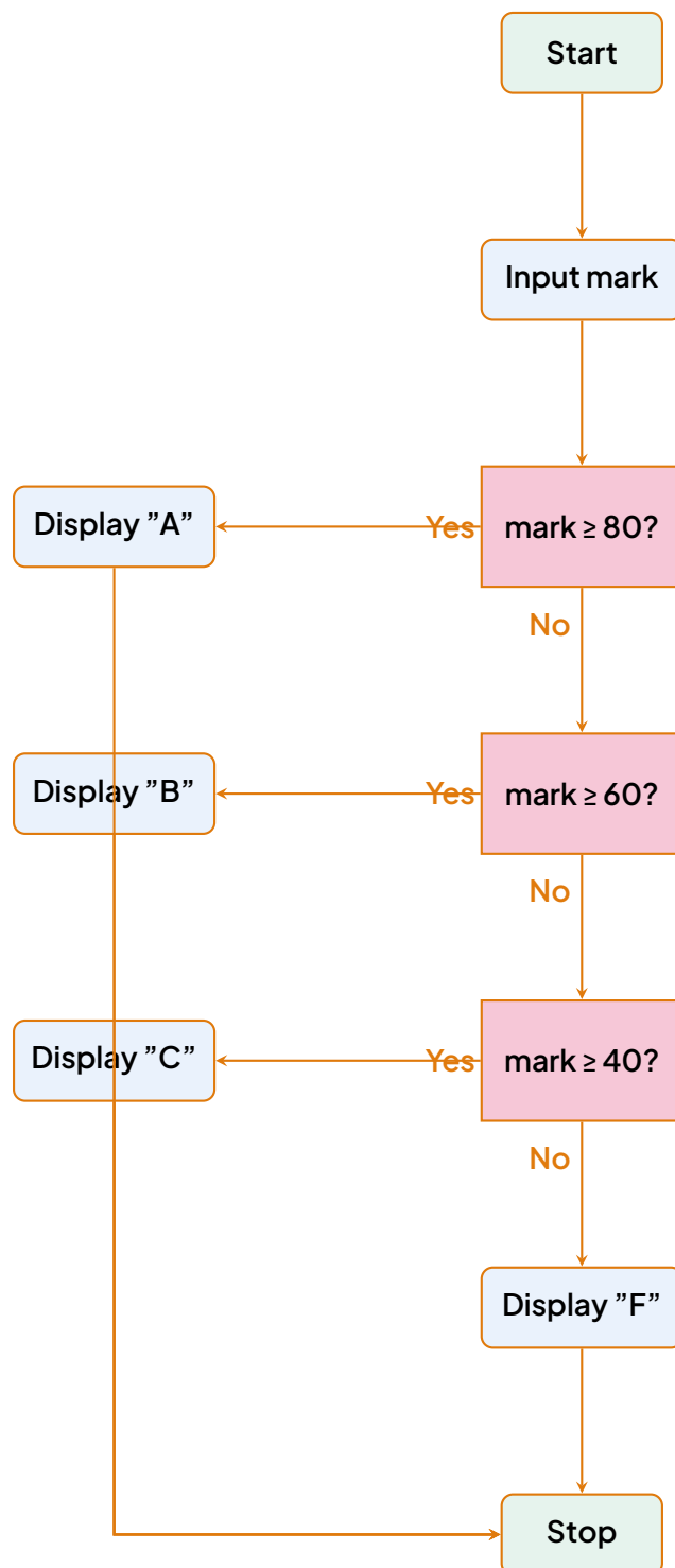
Flowchart for grade determination
