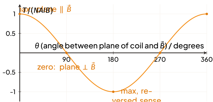
Torque on the coil as a function of the angle \theta between the plane of the coil and the field: T = NAIb \cos \theta .
