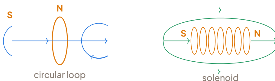
Field patterns of a plane circular loop (left) and a solenoid (right). Outside, the solenoid behaves exactly like a bar magnet; inside, its field is uniform.
