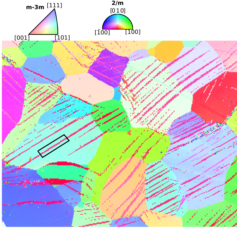
Figure 1: Selection of a region of interest (ROI) on the EBSD orientation map. Austenite grains are coloured by their inverse pole figure (cubic m\bar{3}m key) and the lamellar martensite by the monoclinic 2/m key; the lamellae appear as fine parallel traces inside the parent grains. A single lamella (black rectangle) together with its two interface sides defines the ROI on which the habit-plane analysis is performed.
