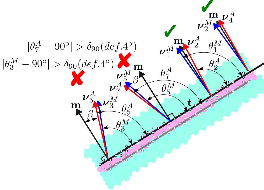
Figure 3: Trace-containment test of Eq. (6), viewed onto the scan surface (plane parallel to the trace). For each phase the candidate plane normals \nu_i^A (red) and \nu_j^M (blue) are projected at points along the trace. A candidate is accepted (✓) when its normal is perpendicular to the trace within tolerance, |\theta^\varphi - 90^\circ| \leq \delta_{90} (default 4^\circ ), with \theta^\varphi = \arccos |\nu^\varphi \cdot \mathbf{t}^\varphi| , and rejected (✗) otherwise. The test is applied independently in austenite ( \varphi = A ) and martensite ( \varphi = M ).
