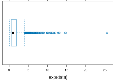
(a) A box plot.
