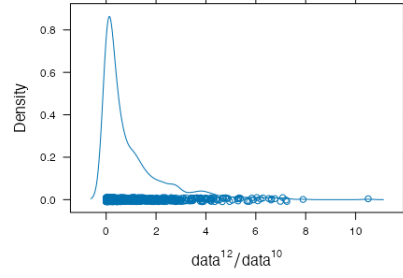
(b) A density plot.
