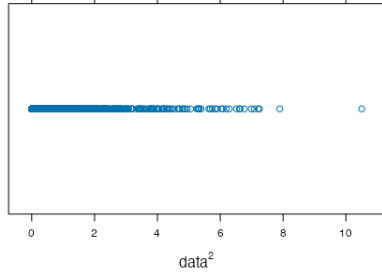
(c) A dot plot.
