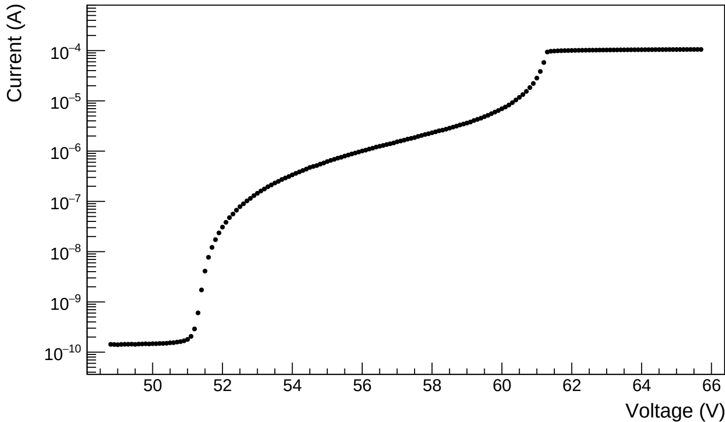
Sensor A1 - 150 °C, 25 h - T = 21\text{ }^{\circ}\text{C}
