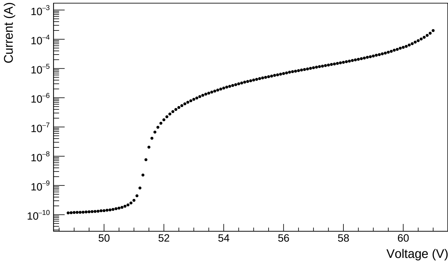
Sensor A1 - 75 °C, 5 h - T = 21^{\circ}\text{C}
