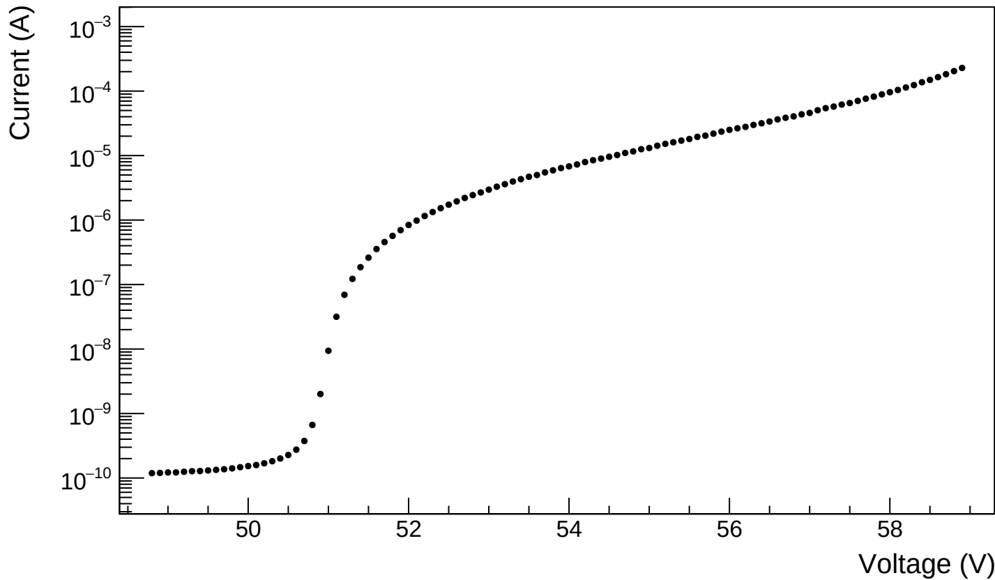
Sensor B1 - 100 °C, 5 h - T = 21^{\circ}\text{C}
