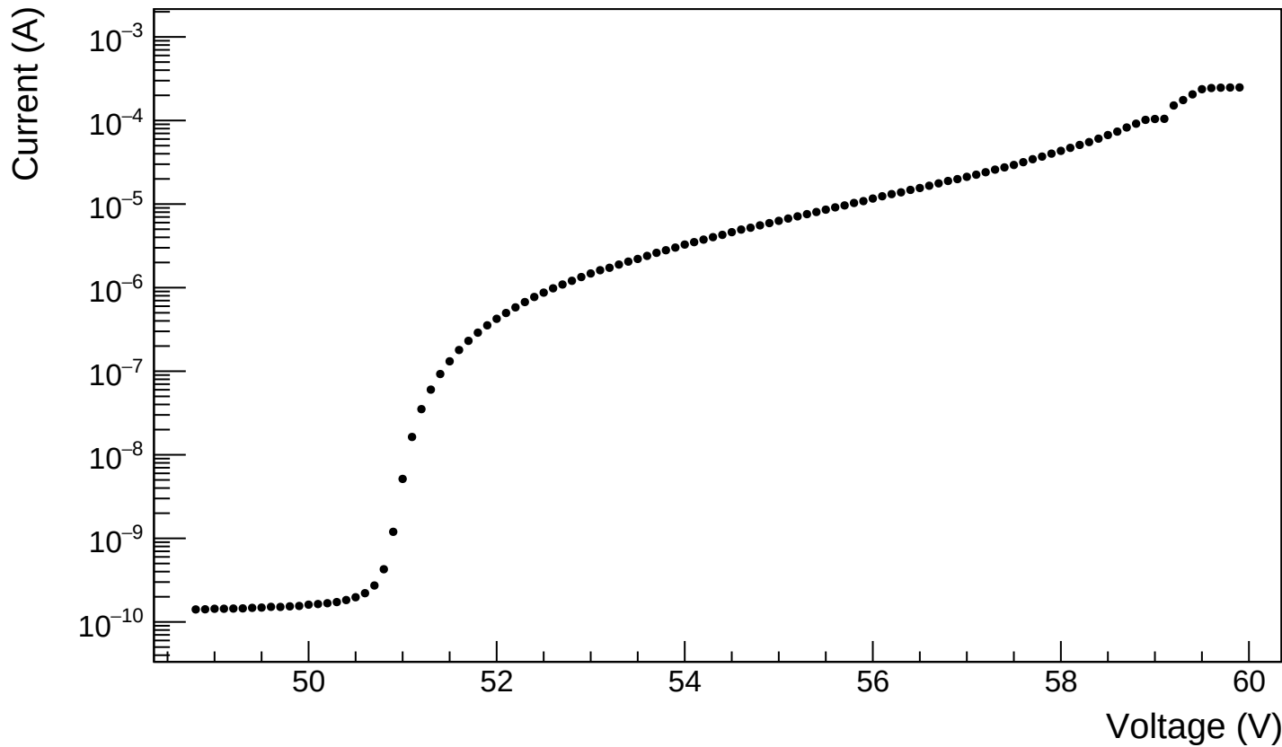
Sensor B1 - 125 °C, 25 h - T = 21 °C
