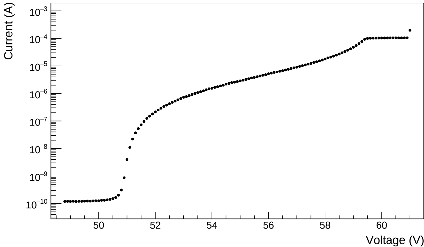
Sensor B1 - 150 °C, 25 h - T = 21^{\circ}\text{C}
