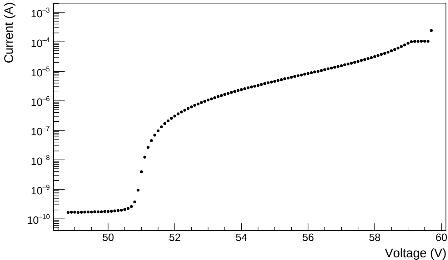
Sensor B1 - 150 °C, 5 h - T = 21^{\circ}\text{C}
