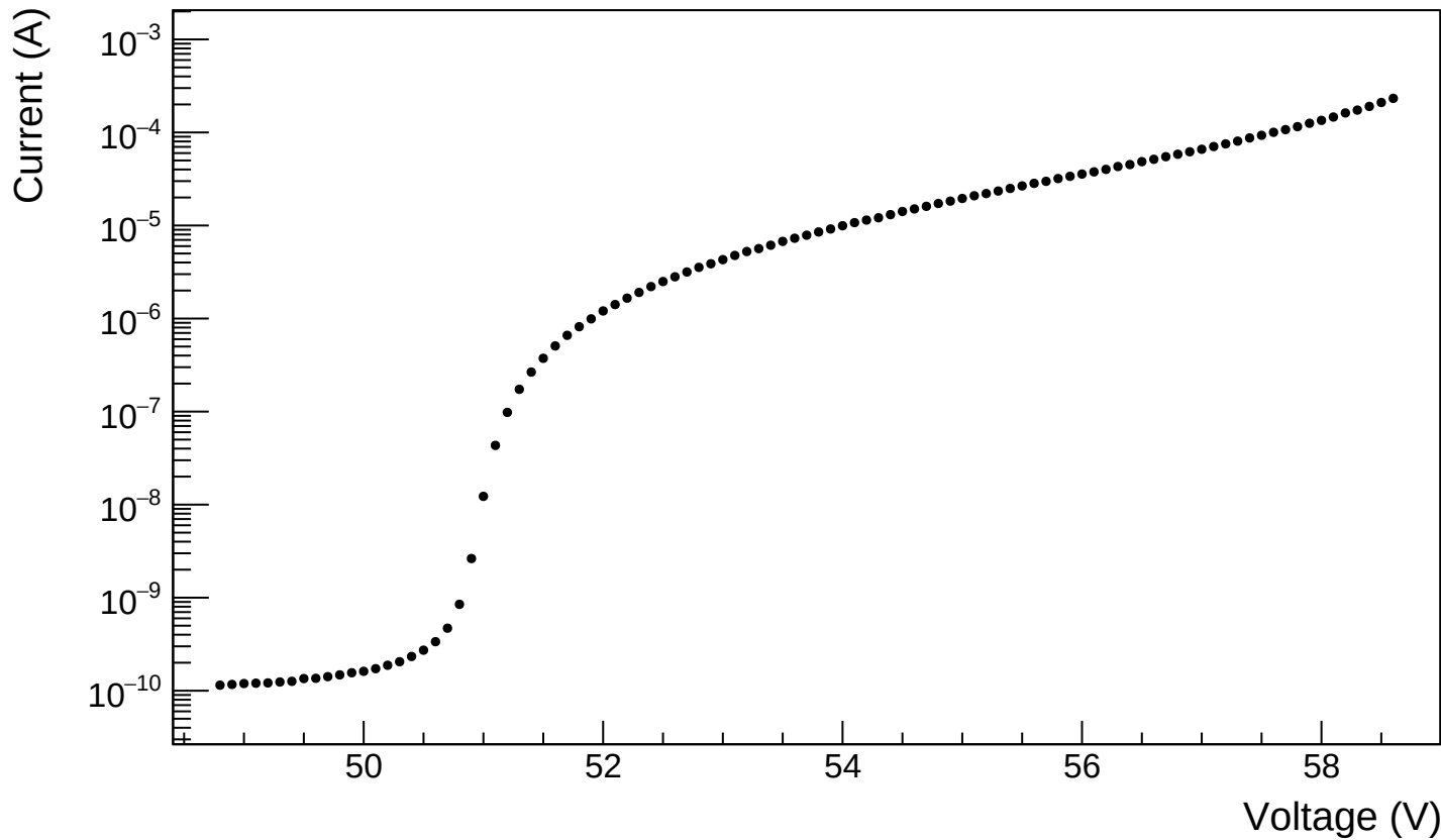
Sensor B1 - 75 °C, 5 h - T = 21 °C
