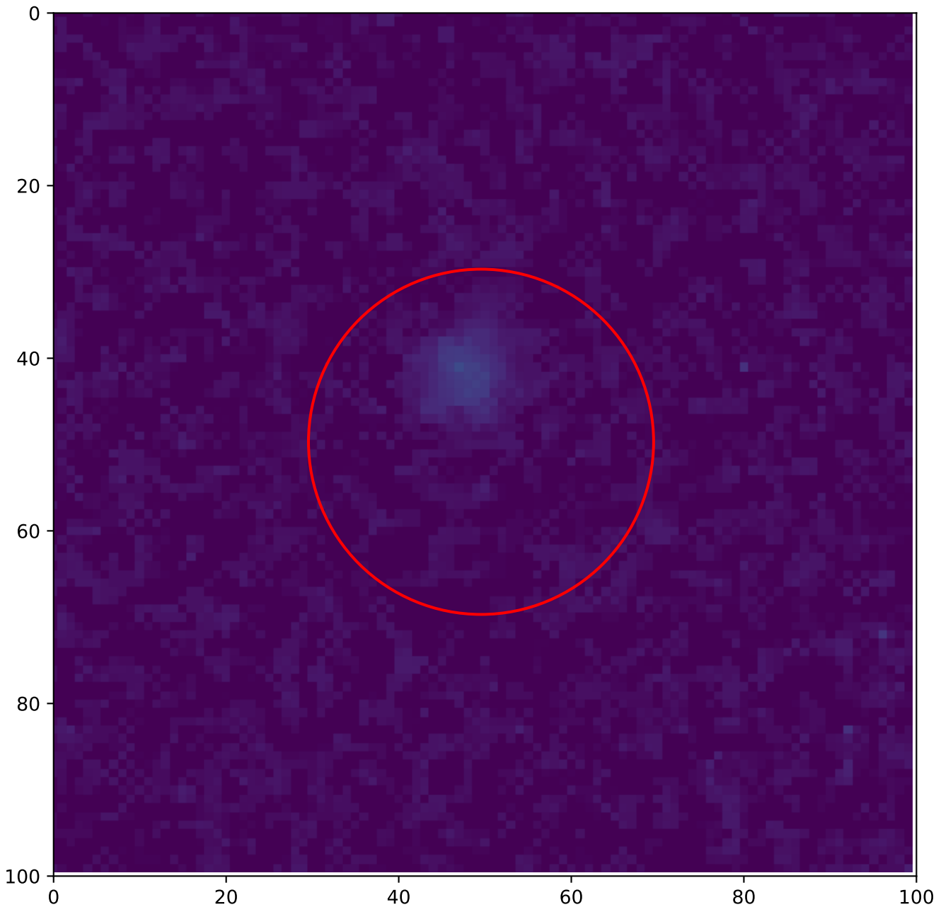
A1 — global hotspot 0 — Annealing 100 °C, 25 h T = 20 °C, v_over = 5 V
