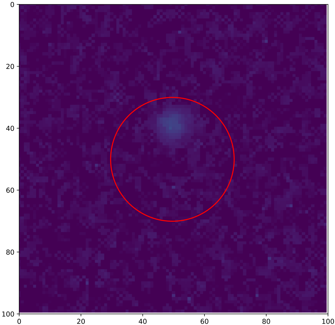
A1 — global hotspot 0 — Annealing 125 °C, 5 h T = 20 °C, v_over = 5 V
