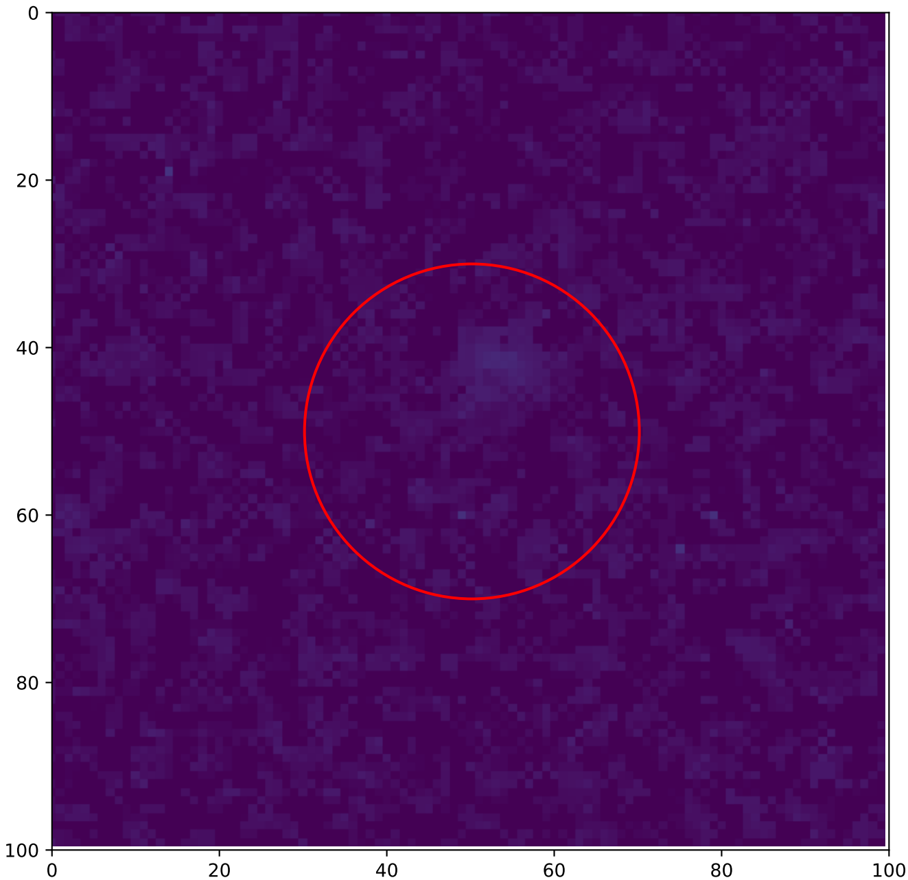
A1 — global hotspot 0 — Annealing 150 °C, 25 h T = 20 °C, v_over = 5 V
