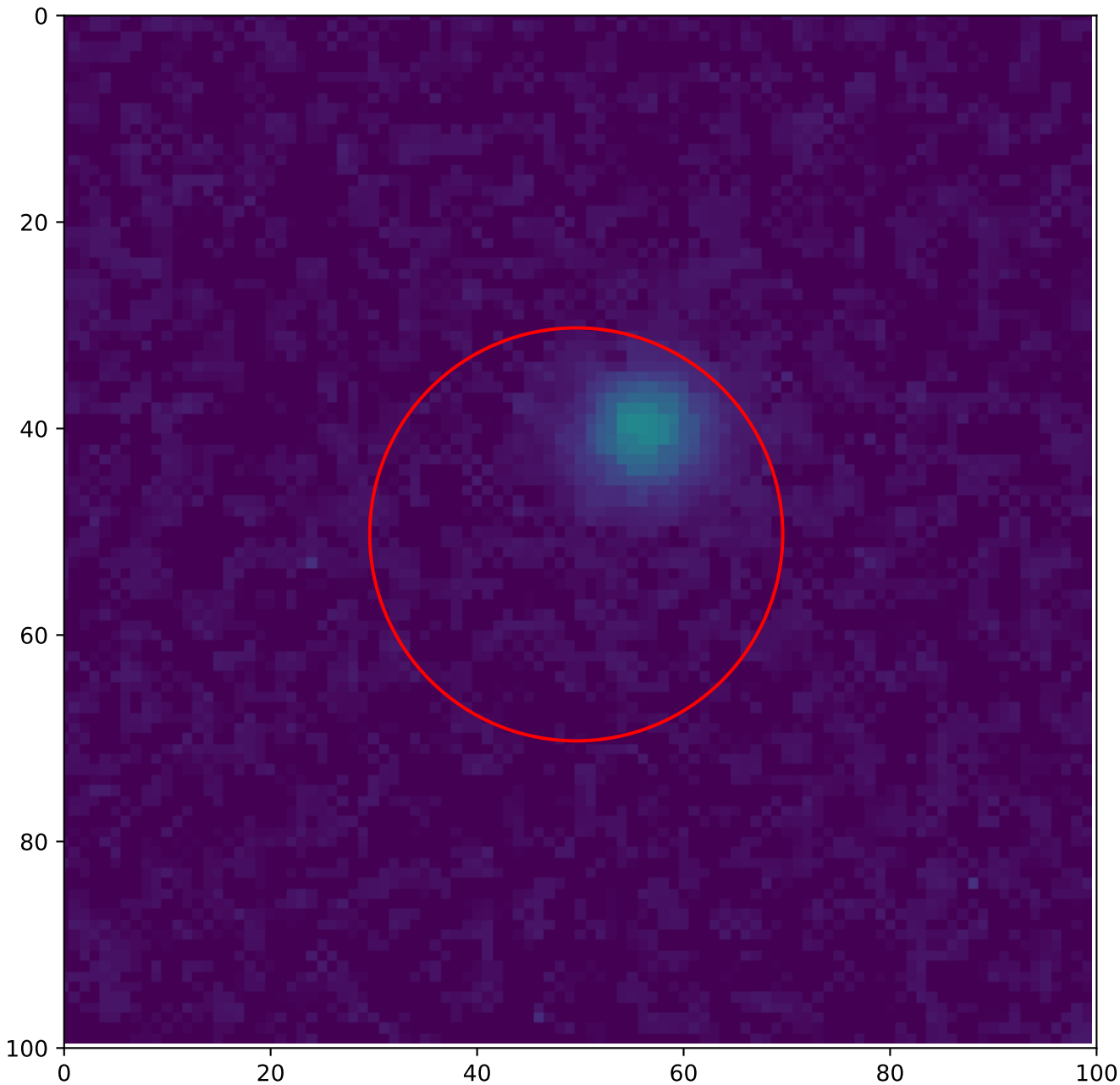
A1 — global hotspot 0 — Annealing 75 °C, 25 h T = 20 °C, v_over = 5 V
