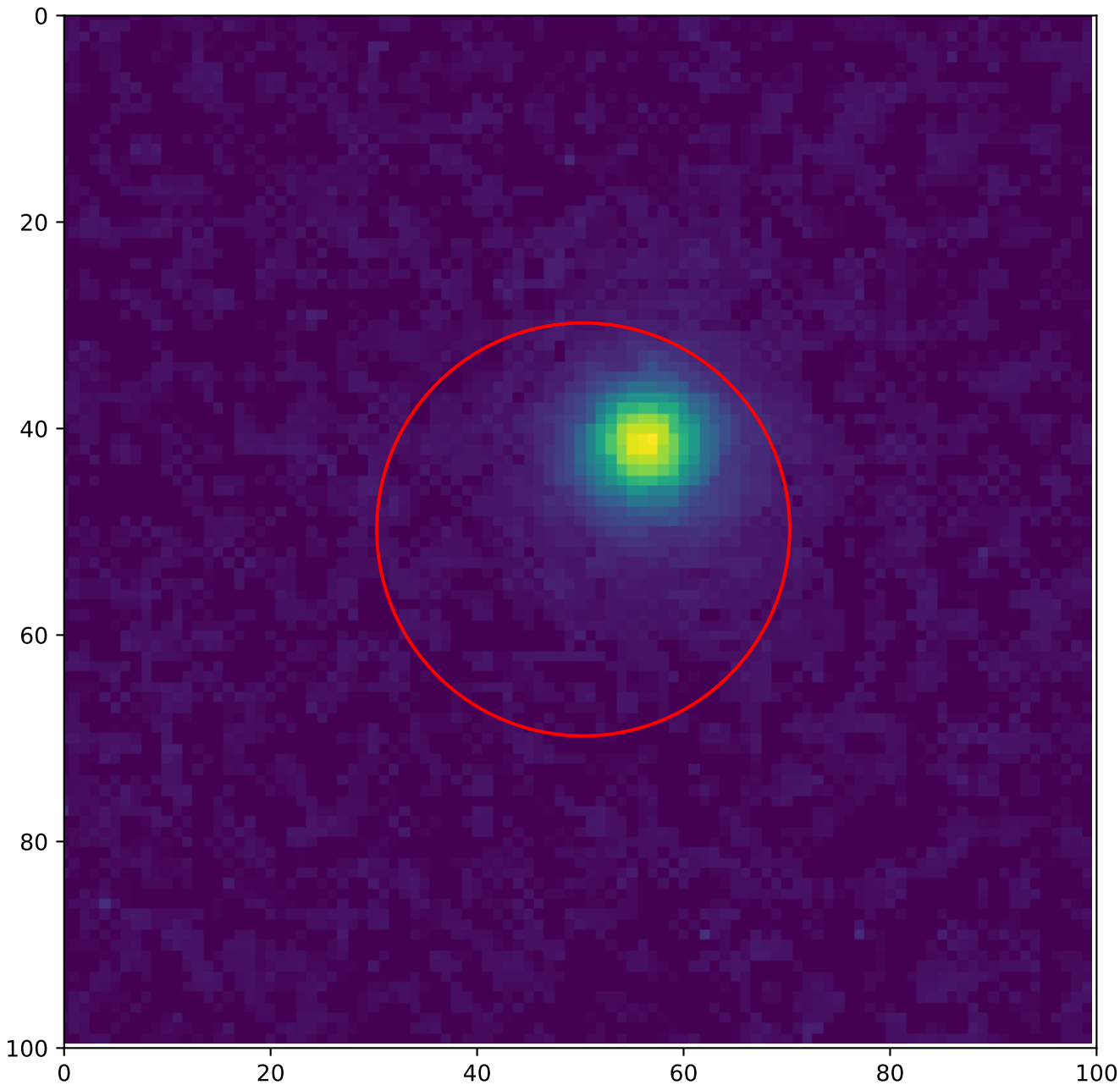
A1 — global hotspot 0 — Annealing 75 °C, 5 h T = 20 °C, v_over = 5 V
