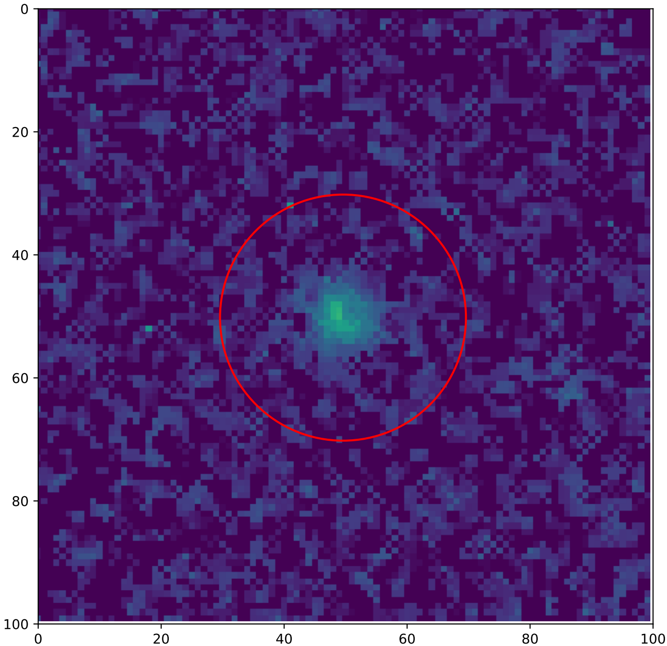
A1 — global hotspot 72 — Annealing 100 °C, 5 h T = 20 °C, v_over = 5 V
