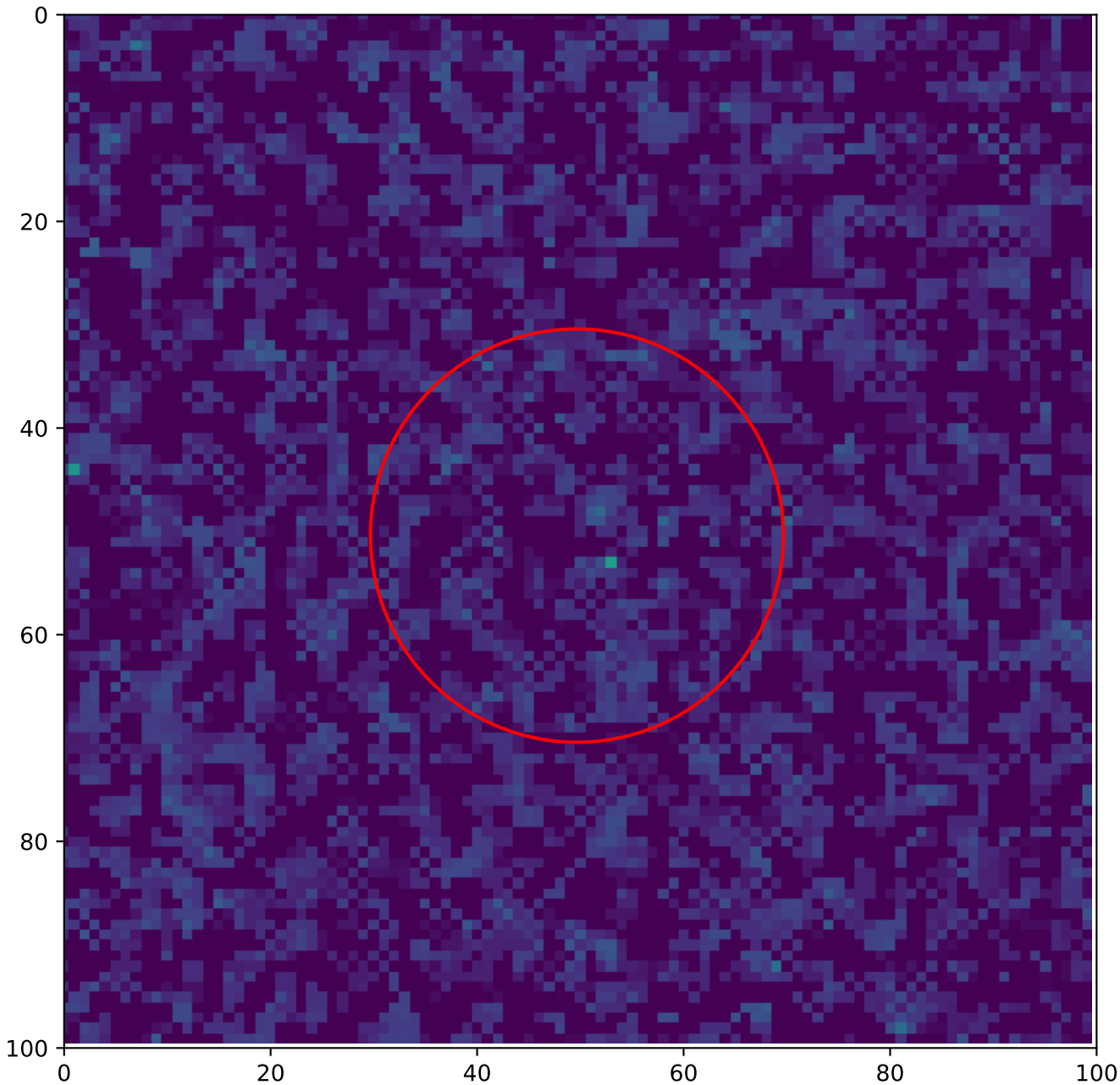
A1 — global hotspot 72 — Annealing 125 °C, 25 h T = 20 °C, v_over = 5 V
