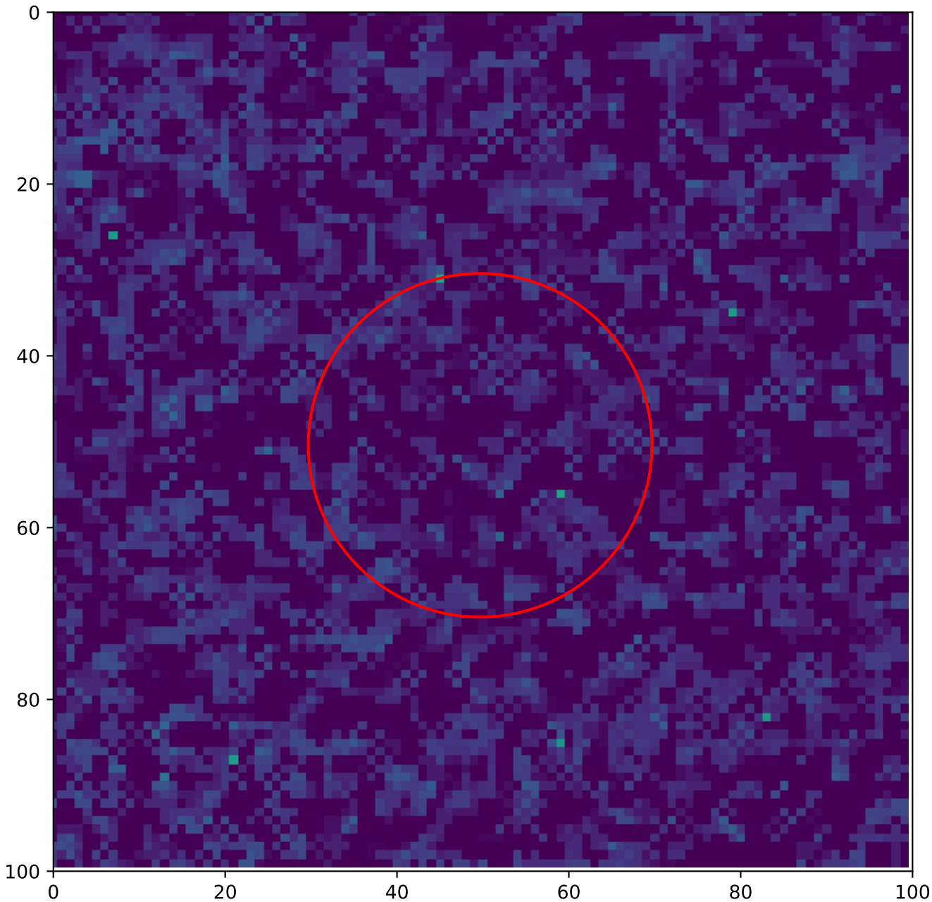
A1 — global hotspot 72 — Annealing 150 °C, 5 h T = 20 °C, v_over = 5 V
