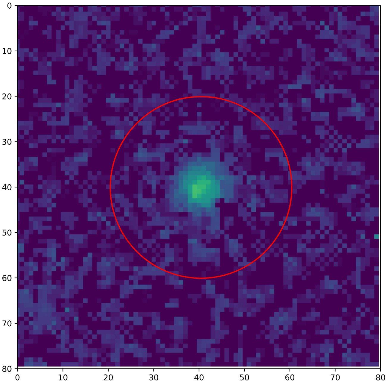
A1 — global hotspot 10 — Annealing 100 °C, 25 h T = 20 °C, v_{\text{over}} = 5 V
