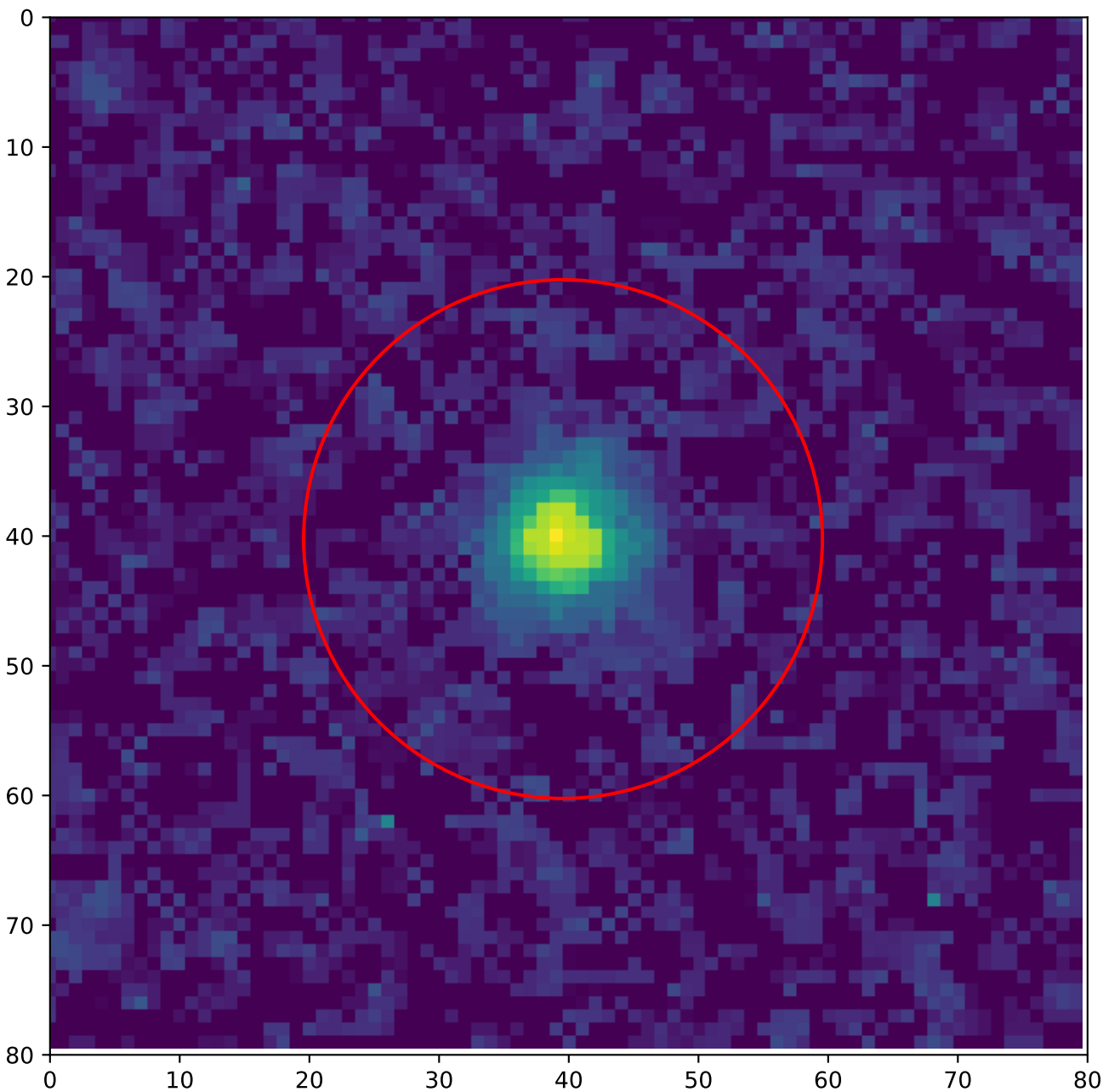
A1 — global hotspot 10 — Annealing 100 °C, 5 h T = 20\text{ °C} , v_{\text{over}} = 5\text{ V}
