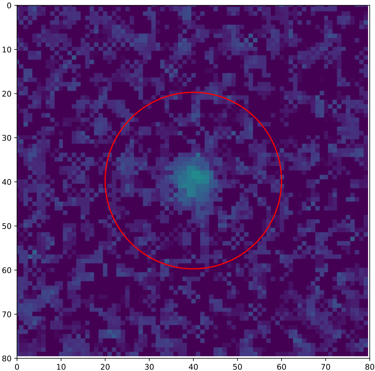
A1 — global hotspot 10 — Annealing 125 °C, 25 h T = 20 °C, v_{\text{over}} = 5 V
