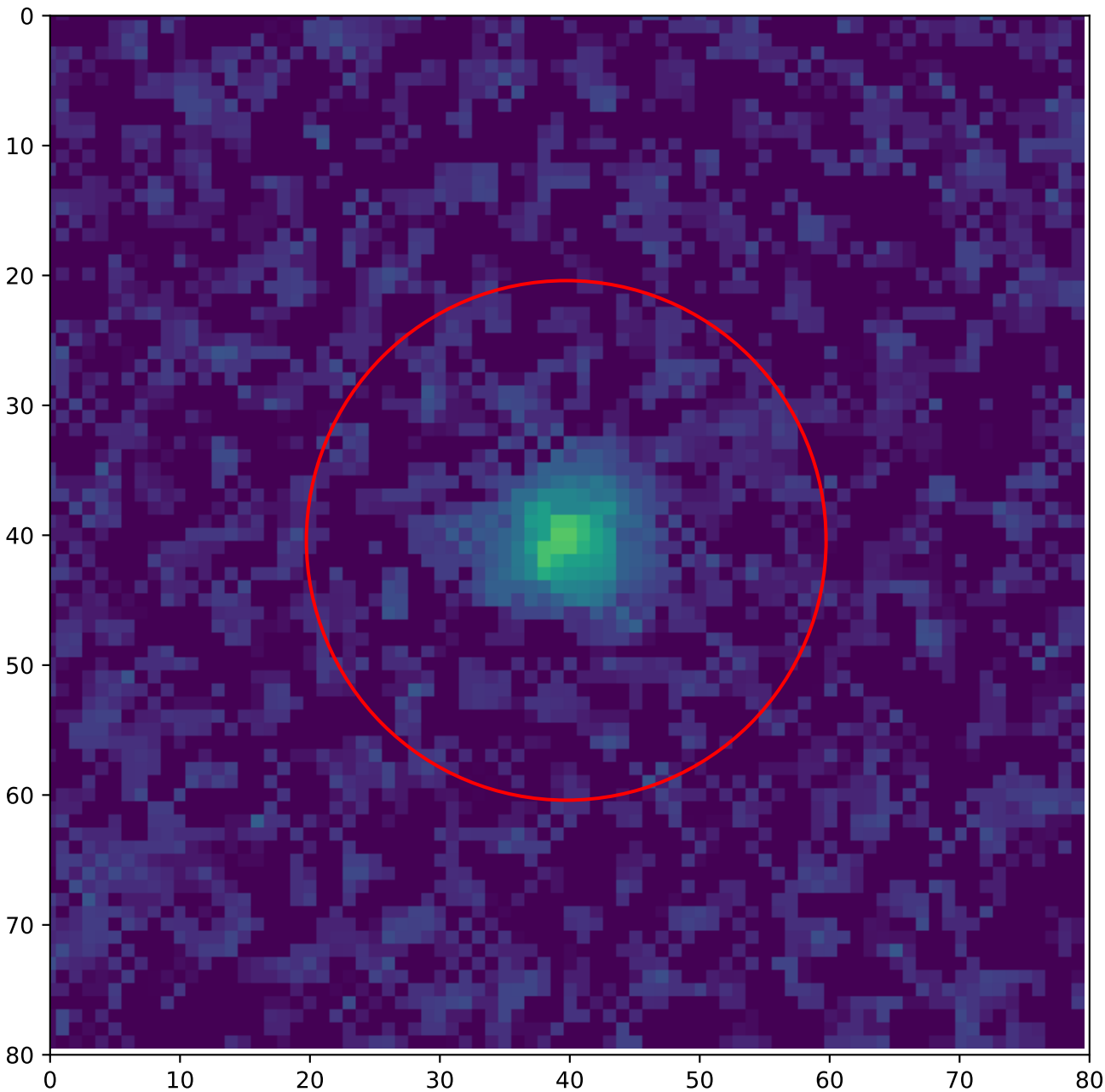
A1 — global hotspot 10 — Annealing 125 °C, 5 h T = 20 °C, v_{\text{over}} = 5 V
