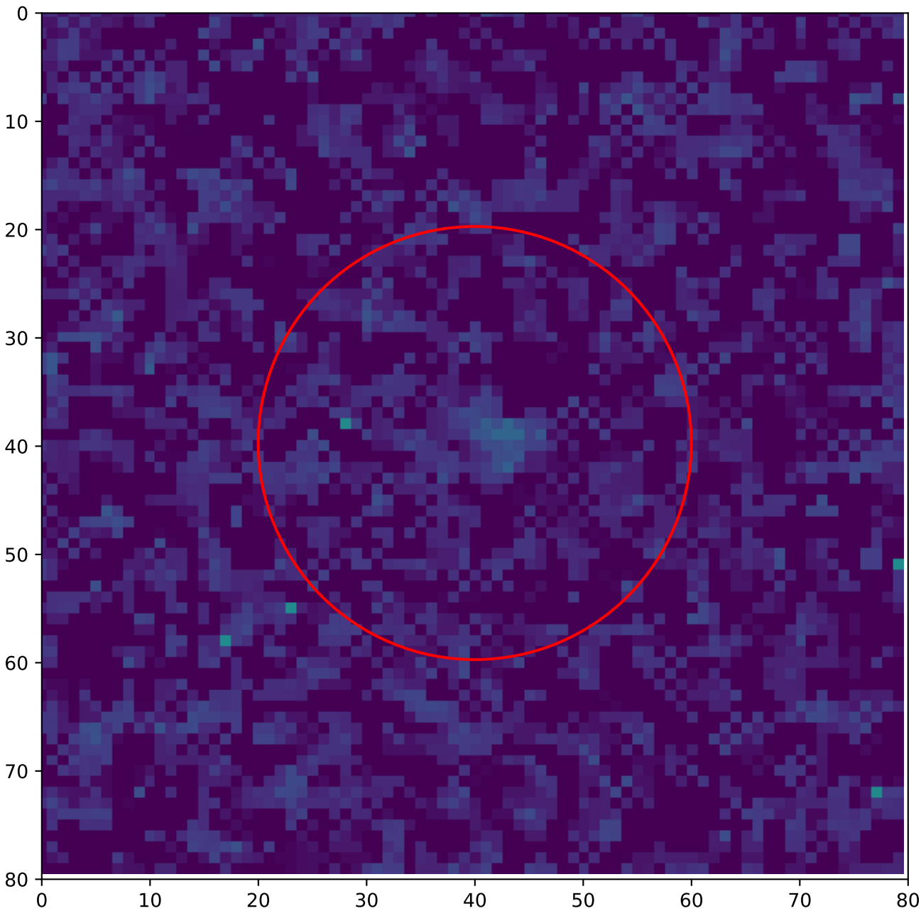
A1 — global hotspot 10 — Annealing 150 °C, 5 h T = 20 °C, v over = 5 V
