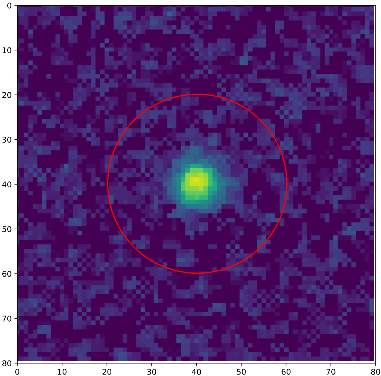
A1 — global hotspot 10 — Annealing 75 °C, 25 h T = 20 °C, v over = 5 V
