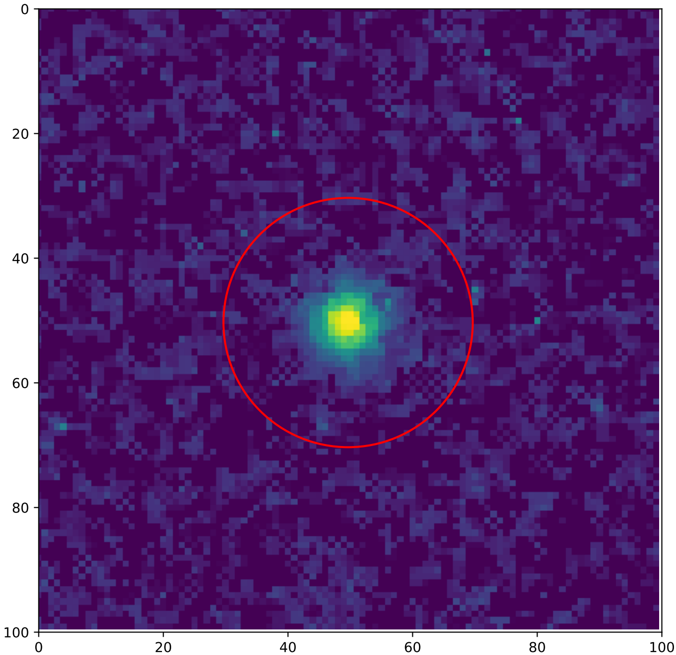
A1 — global hotspot 4 — Before annealing T = 20\text{ }^{\circ}\text{C} , v_{\text{over}} = 5\text{ V}
