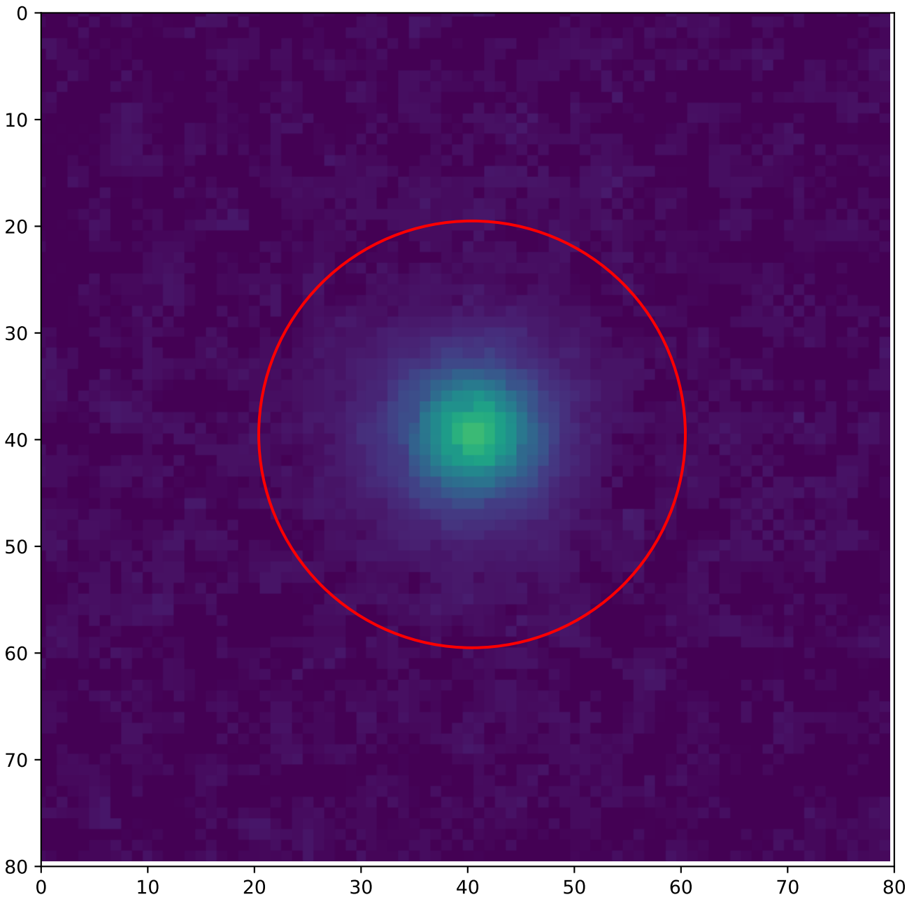
A1 — global hotspot 54 — Annealing 100 °C, 25 h T = 20 °C, v_{\text{over}} = 5 V
