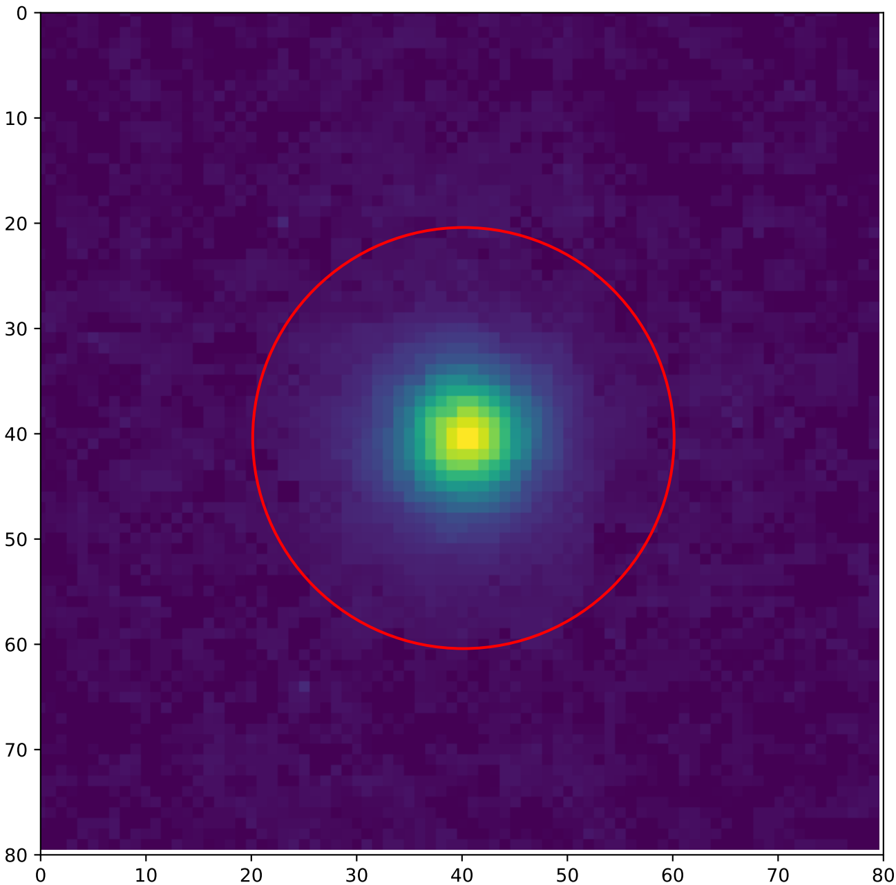
A1 — global hotspot 54 — Annealing 75 °C, 25 h T = 20 °C, v_over = 5 V
