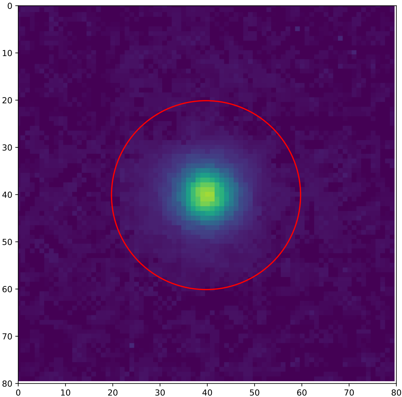
A1 — global hotspot 54 — Annealing 75 °C, 5 h T = 20 °C, v over = 5 V
