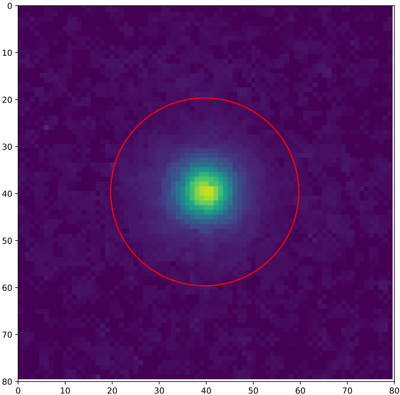
A1 — global hotspot 54 — Before annealing T = 20\text{ }^{\circ}\text{C} , v_{\text{over}} = 5\text{ V}
