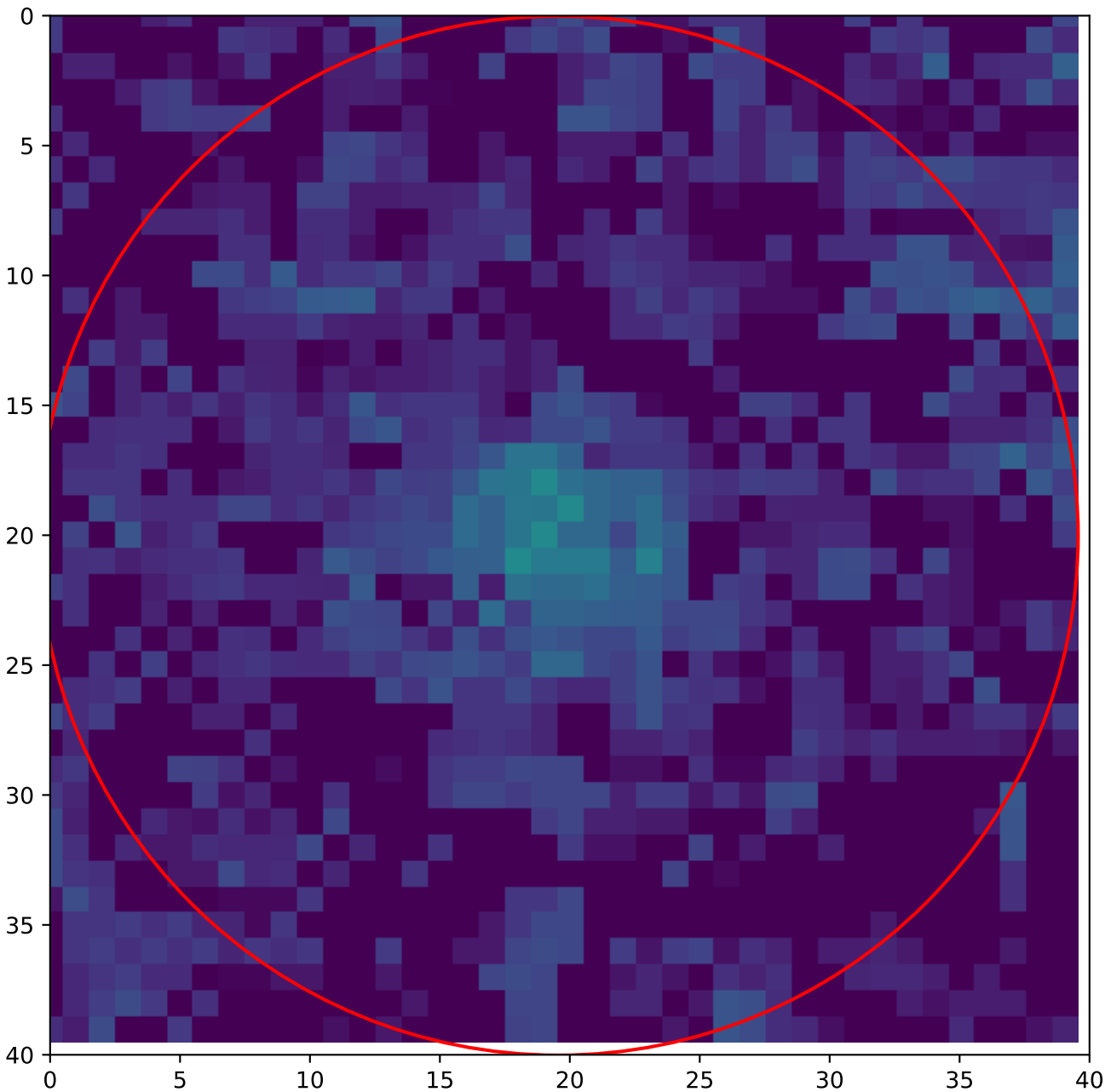
A1 — global hotspot 72 — Annealing 100 °C, 25 h T = 20 °C, v over = 5 V
